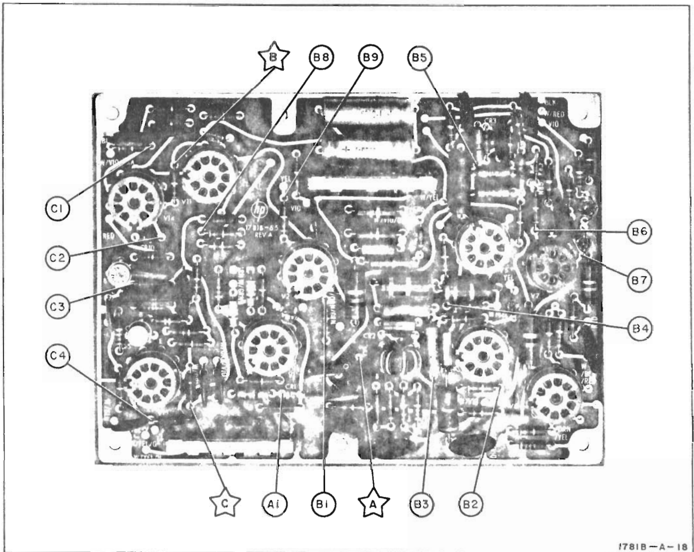
Figure 5-2. Location of Test Points
