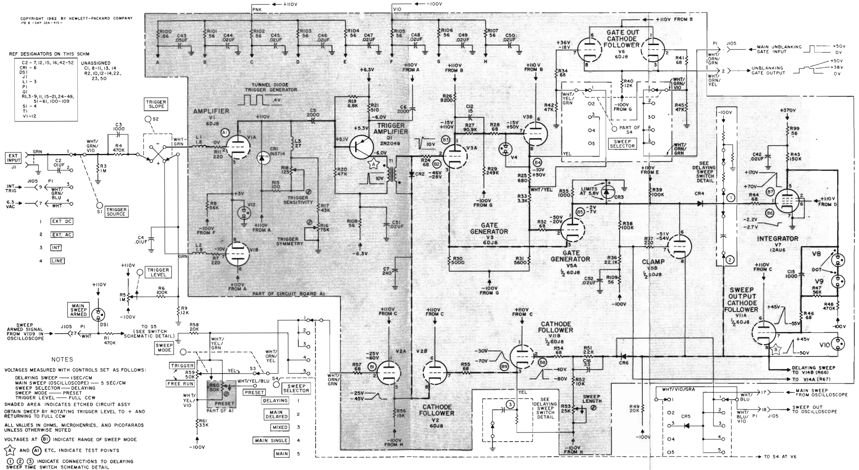
Figure 5-9. Sweep Generator 5-15
