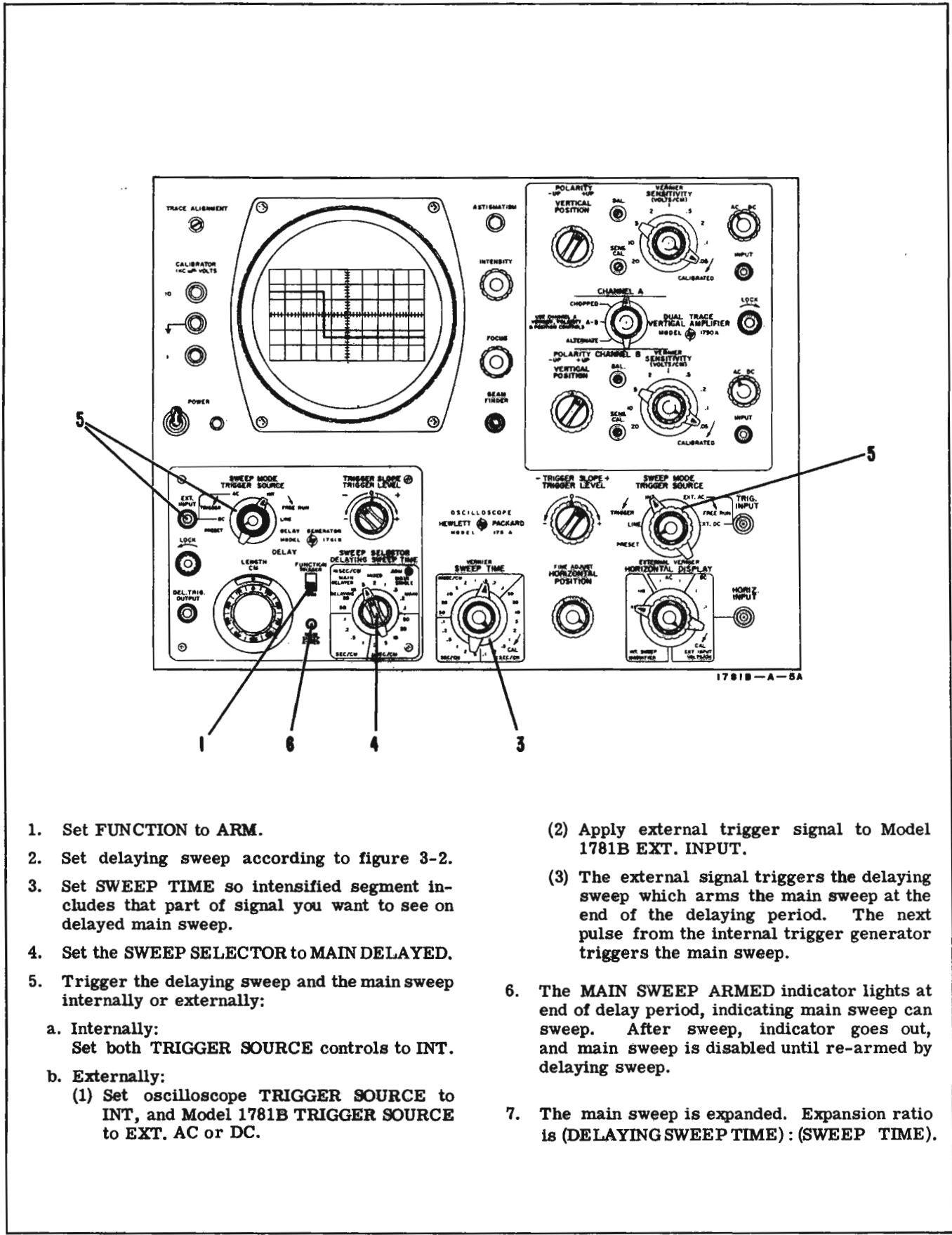
Figure 3-4. Main Sweep, Delayed and Armed
