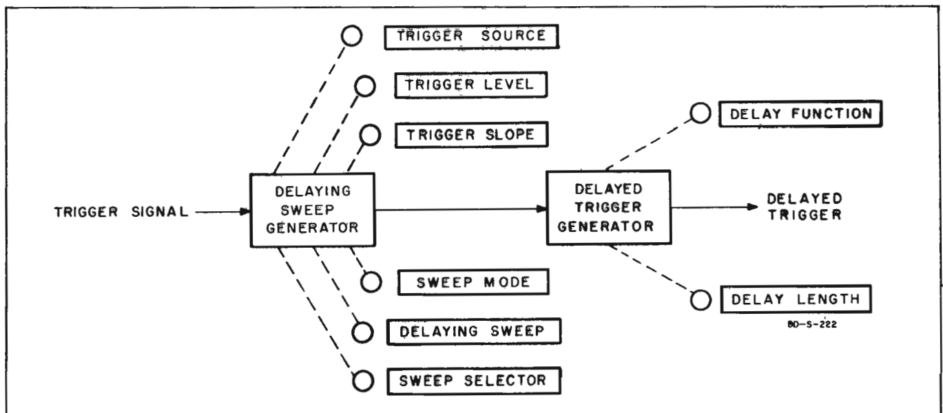
Figure 4-1. Overall Block Diagram
